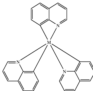
[Chemical Formula 2]
