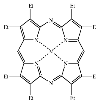
[Chemical Formula 1]
